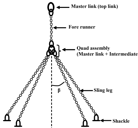
Figure E-1 Four legged Chain Sling Lifting Sling with Fore runner
